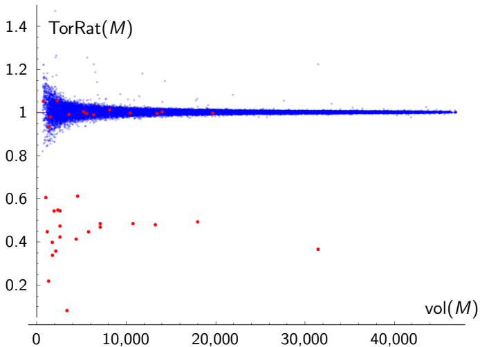
Covers of nonarithmetic twist-knot orbifolds.
